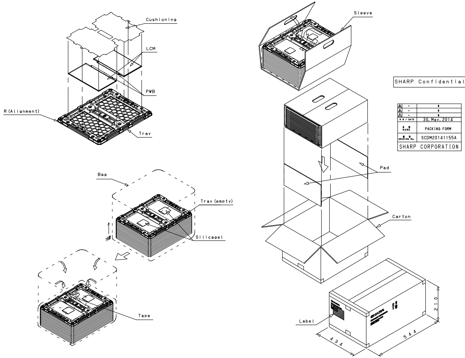
Fig. 1 Packing Condition
