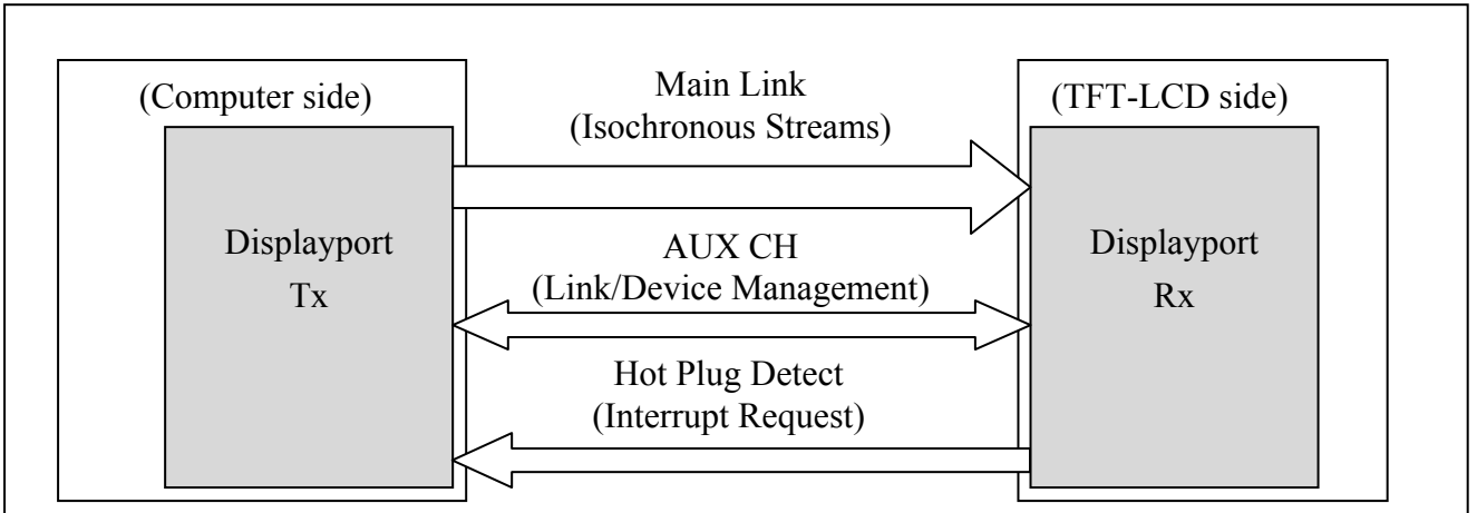
Fig.4-2-1 DP architecture.
